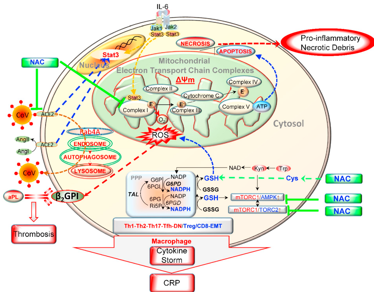
Fig. 3. Schematic diagram of metabolic pathways that control oxidative stress and mTOR-dependent generation of cytokine storm. The depicted surface receptors and transducers exemplify those that operate in T cells and underlie pro-inflammatory lineage development as well as hepatocytes that secrete apolipoprotein H, also known as \beta 2-glycoprotein I ( \beta 2GPI). Oxidized \beta 2GPI is the primary antigen that elicits the formation of antiphospholipid antibodies (aPL) in patients with antiphospholipid syndrome [22]. Thus, oxidation of \beta 2GPI induces not only aPL but also promotes cardiovascular disease [24] in the setting of COVID-19 infection [25–27]. IL-6, the primary cytokine that drives inflammation in COVID-19 infected patients, elicits mitochondrial oxidative stress at complex I of the mitochondrial electron transport chain (ETC). In turn, this leads to redox-dependent activation of mTORC1. Further downstream, uncontrolled activation of mTORC1 promotes inflammation [28]. NAC inhibits oxidative stress by serving as a cell-permeable amino acid precursor of the main intracellular antioxidant, GSH. Acting outside the cell, NAC may break disulfide bonds within ACE2 that serves as the cellular receptor for COVID-19 [15]. NAC may also block COVID-19 binding by disrupting disulfide bond within its receptor-binding domain [29]. In addition to epithelial, endothelial, and myocardial cells [30,31], ACE2 is expressed on T lymphocytes [32], macrophages [33], and hepatocytes [34–37]. ACE2 controls the expression of pro-inflammatory transcription factor Stat3 [38–43], which also modulates the production of reactive oxygen intermediates by complex I of the mitochondrial electron transport chain (ETC) [44]. ACE2 also attenuates signaling through mTORC1 [45–48].
